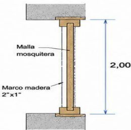
CORTE VERTICAL
